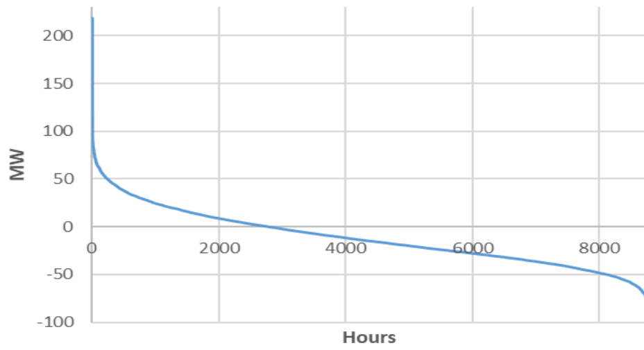
Monotone curve for compensation deficit 2023 380-220-150 kV network
